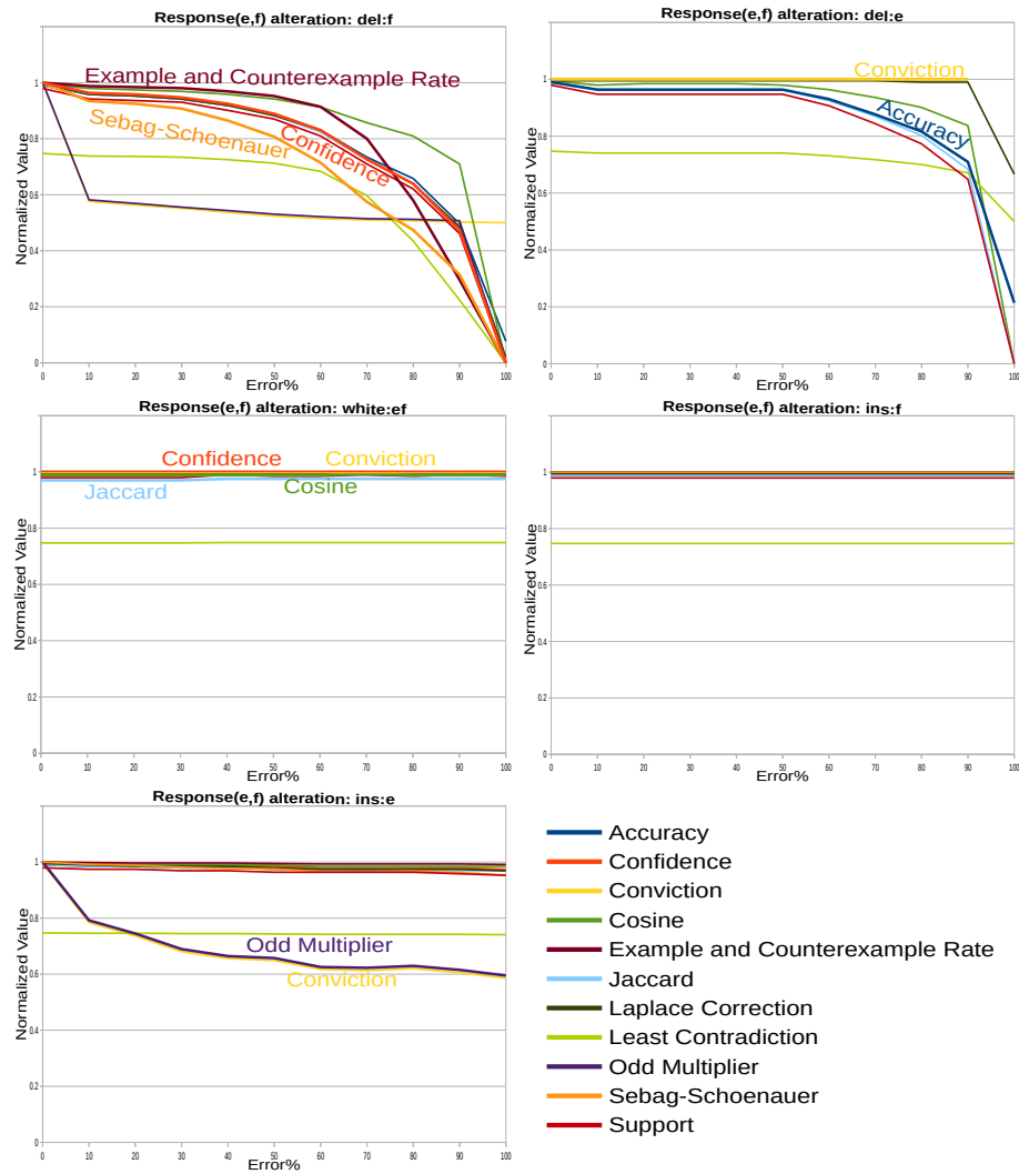
Figure 5: Effect of error injection on constraint \text{RESPONSE}(e, f) for the best 10 scoring measures from the ranking experiment in Section 6.1.
