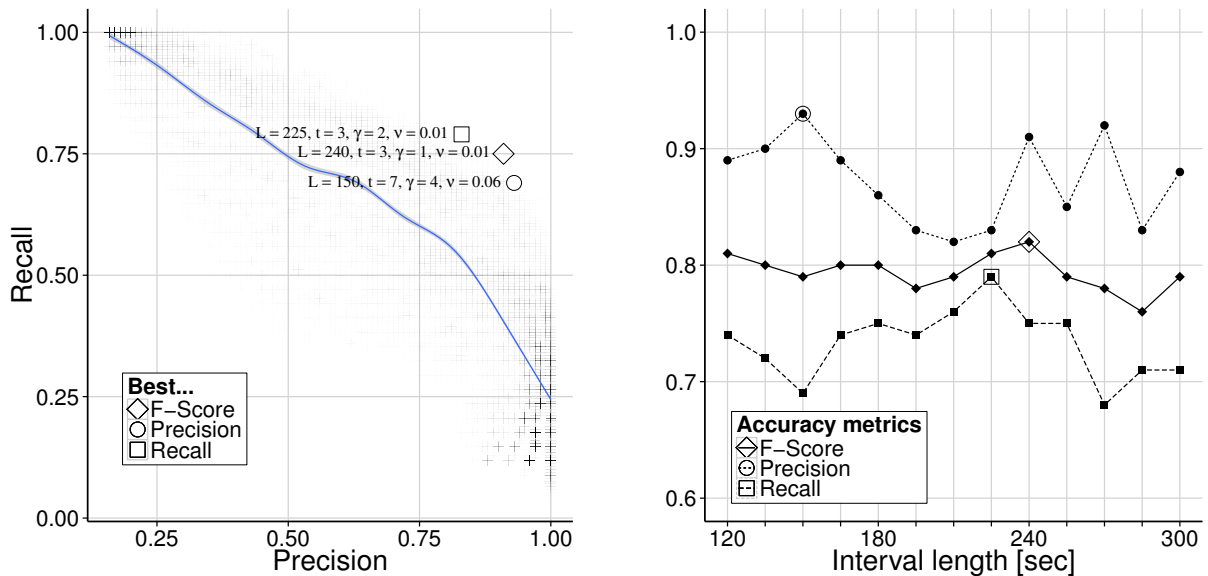
(a) Precision-recall graph for the validation phase of the SVM. (b) The trend of best F-score values gained in the validation phase of the SVM with respect to the interval length, and the corresponding precision and recall.
